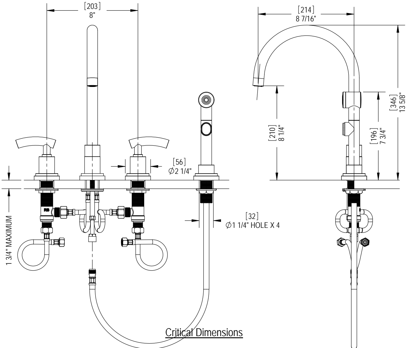
H2O Widespread Kitchen Set with Hand Spray Model: 8BRBHOL XX-XX
